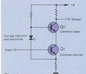
Fig. 1 Basic Circuit of the Cascode Connection Amplifier
